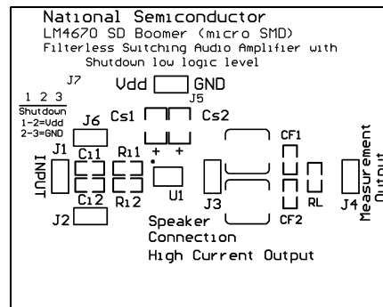
Figure 40. Silk Screen
