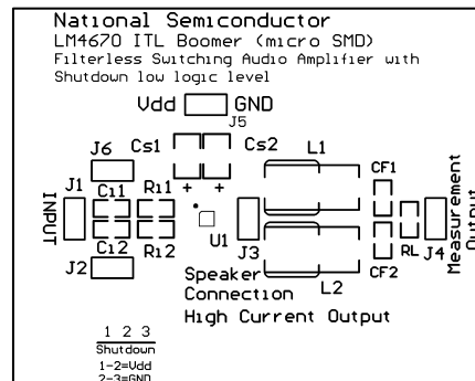
Figure 34. Silk Screen
