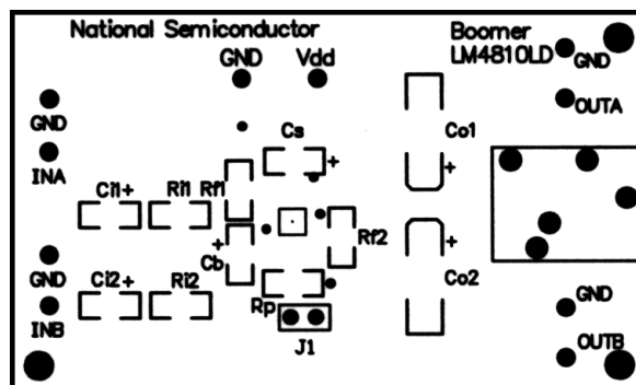
Figure 45. Recommended NGL0008B PC Board Layout Component-Side Silkscreen
