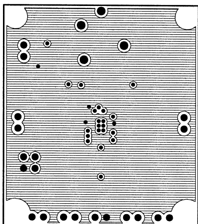
Figure 53. Recommended LQ PC Board Layout: Upper Inner-Layer Layout
