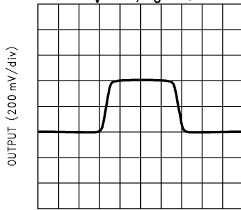
TIME (20 ns/div) Figure 40.
