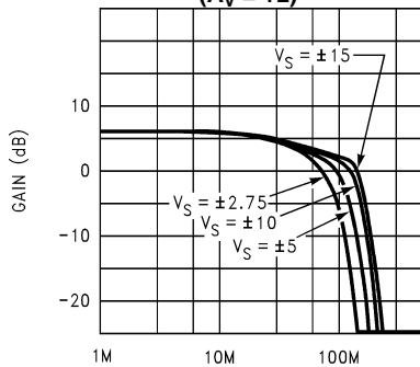
FREQUENCY (Hz) Figure 42.
