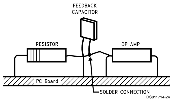
FIGURE 11. Air Wiring
