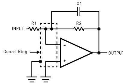
Figure 33. Inverting Amplifier
