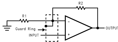
Figure 34. Non-Inverting Amplifier
