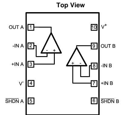
Figure 3. 10-Pin VSSOP Package See Package Number DGS0010A
