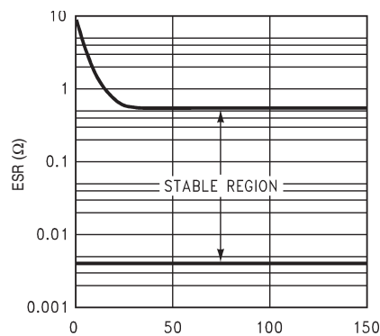
Figure 32. 2.2- \mu\text{F} /3.3- \mu\text{F} Stable ESR Range for Output Voltage \geq 2.5\text{ V}
