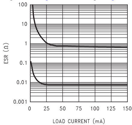
Figure 30. 2.2- \mu\text{F} Stable ESR Range for Output Voltage \leq 2.3\text{ V}
