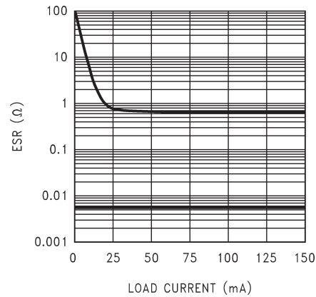
Figure 31. 4.7- \mu\text{F} Stable ESR Range for Output Voltage \leq 2.3\text{ V}
