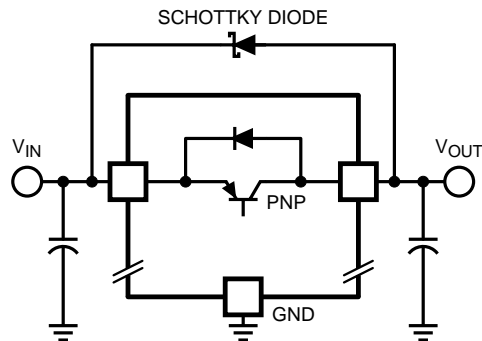
Figure 38. Operation with Schottky Diode
