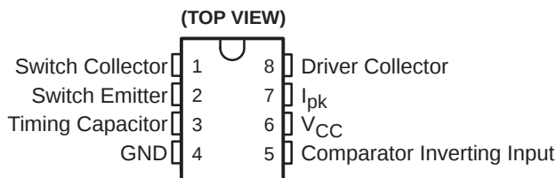
D (SOIC) OR P (PDIP) PACKAGE
