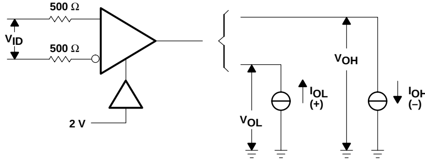
Figure 1. V_{OH} , V_{OL}
