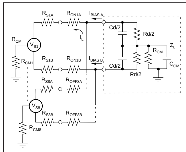
FIGURE 2. MPC507A Static Accuracy Equivalent Circuit.
