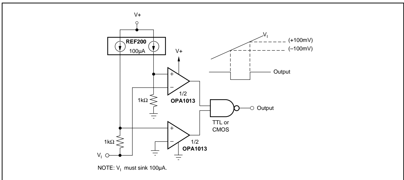
FIGURE 4. Window Comparator.
