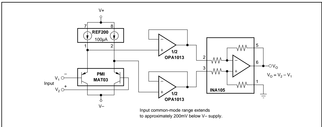
FIGURE 3. Instrumentation Amplifier.
