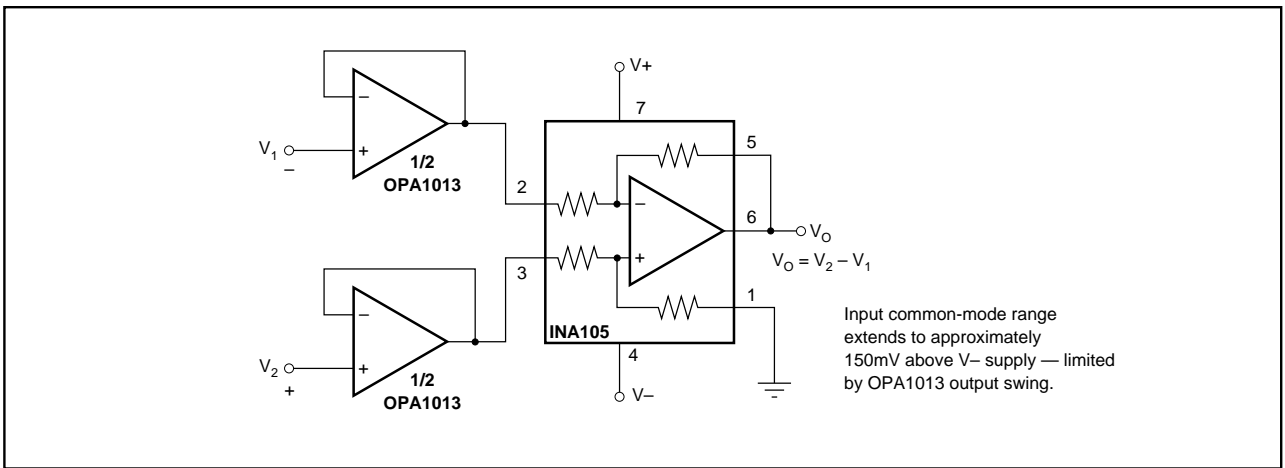
FIGURE 2. Instrumentation Amplifier.
