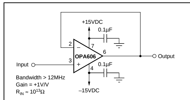
FIGURE 5. Noninverting Buffer.
