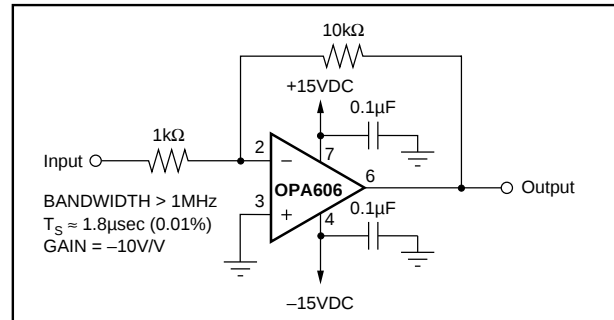
FIGURE 4. Inverting Amplifier.
