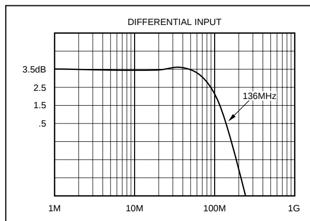
FIGURE 10. Measured Frequency Response for INA.
