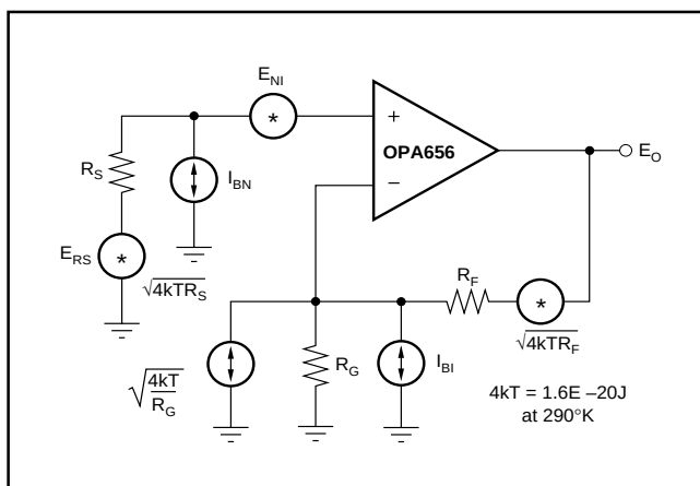
The total output spot noise voltage can be computed as the square root of the squared contributing terms to the output noise voltage. This computation is adding all the contributing noise powers at the output by superposition, then taking the square root to get back to a spot noise voltage. Equation 1 shows the general form for this output noise voltage using the terms shown in Figure 4.
