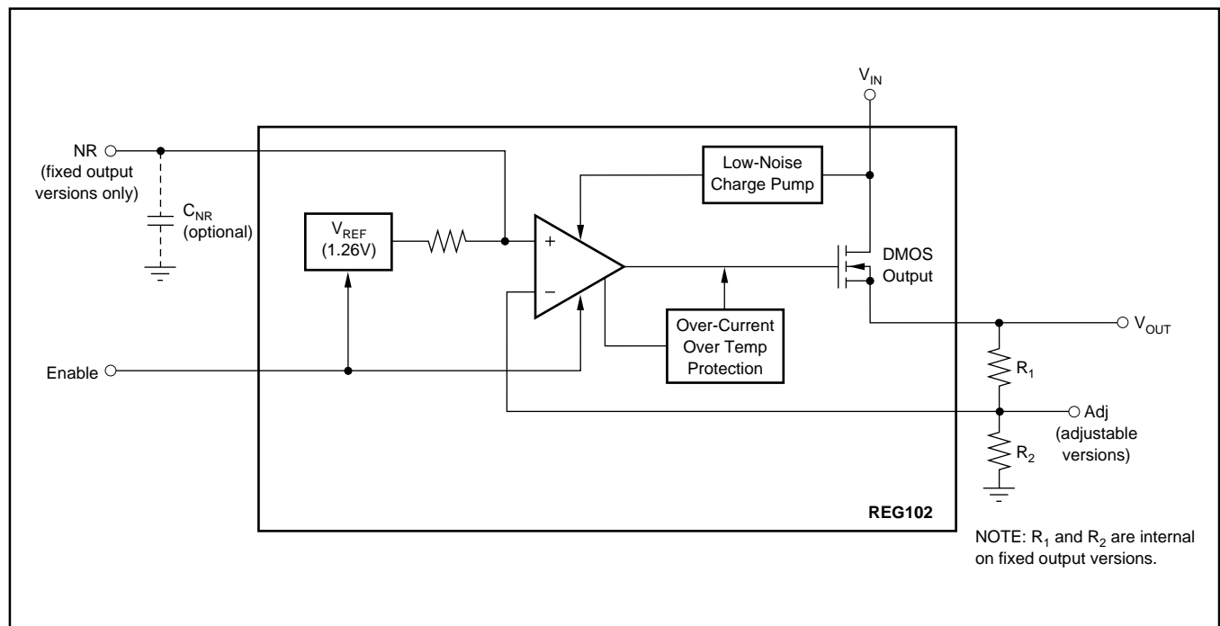
FIGURE 4. Block Diagram.
