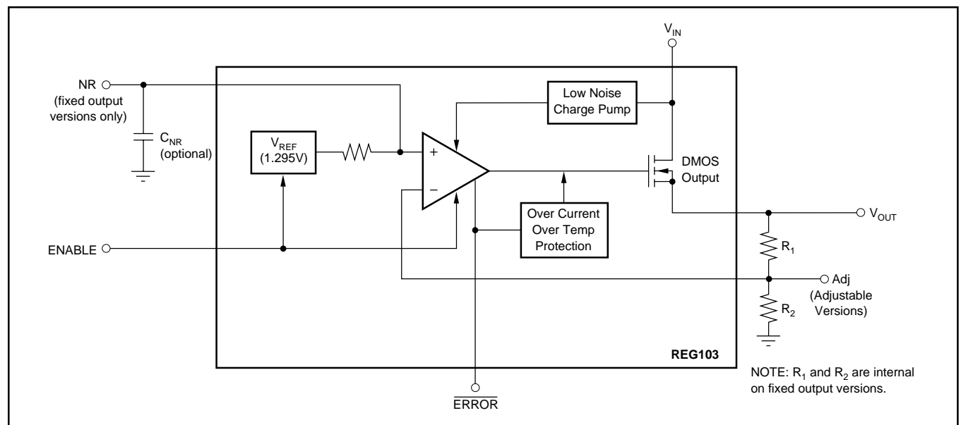
FIGURE 7. Block Diagram.
