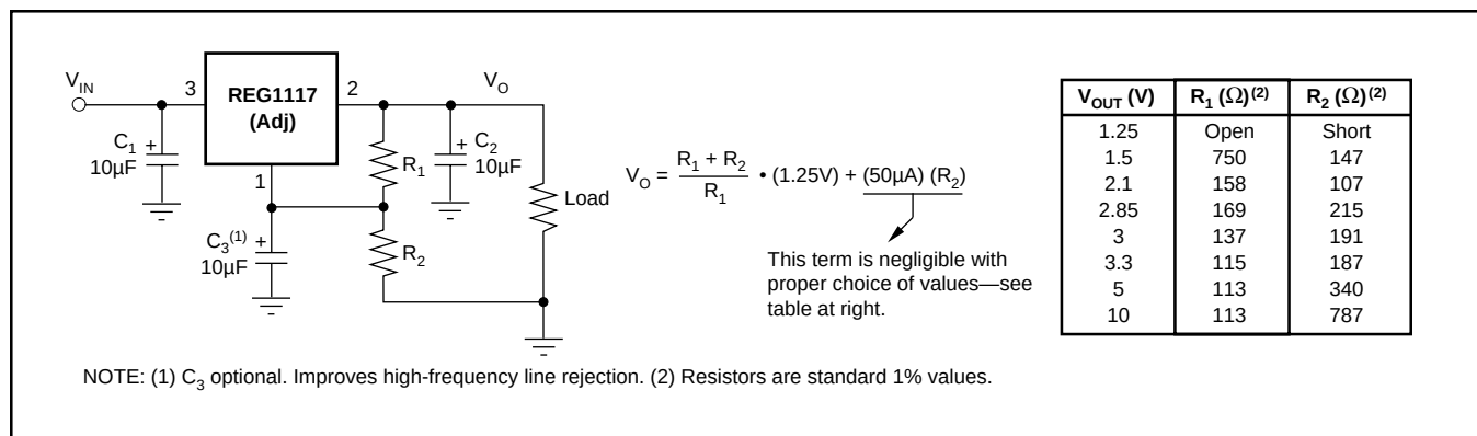
FIGURE 2. Adjustable-Voltage Model—Basic Connections.
