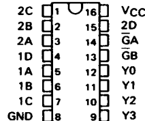
SN54285 . . . J OR W PACKAGE SN74285 . . . N PACKAGE (TOP VIEW)
