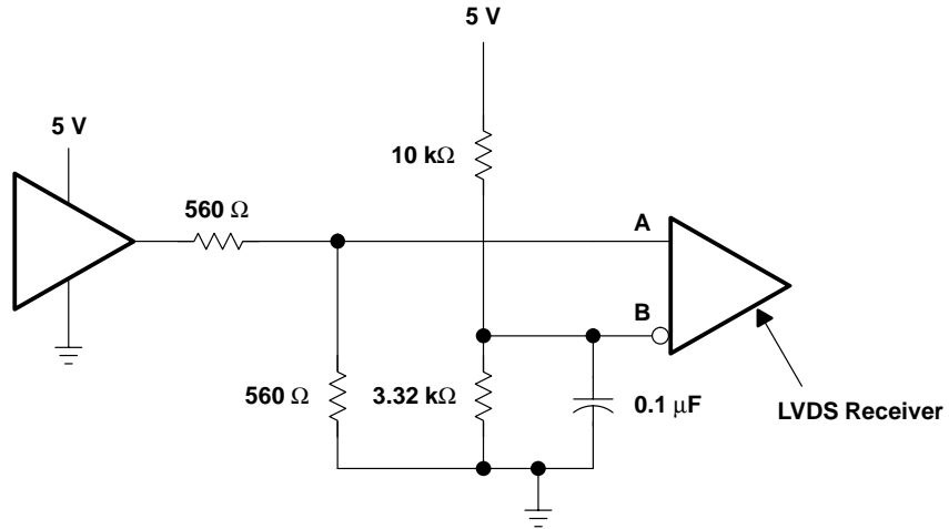
Figure 19. 5-V CMOS
