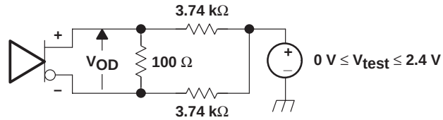
Figure 7. V_{OD} Test Circuit
