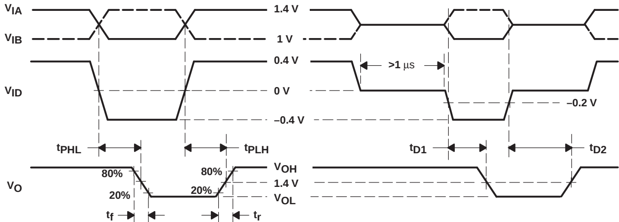
Figure 3. Timing Test Circuit and Waveforms
