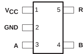
SN65LVDT2 DBV PACKAGE (TOP VIEW)
