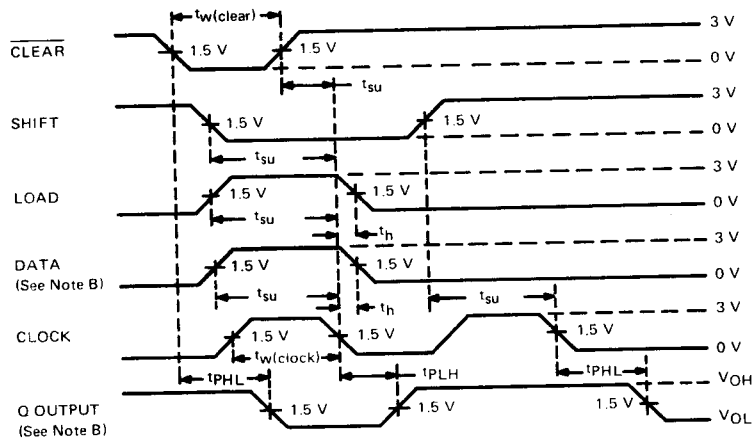
VOLTAGE WAVEFORMS
