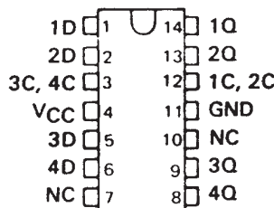
SN5477, SN54LS77 . . . W PACKAGE (TOP VIEW)
