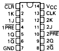
SN54HC114 ... J PACKAGE SN74HC114 ... D OR N PACKAGE (TOP VIEW)
