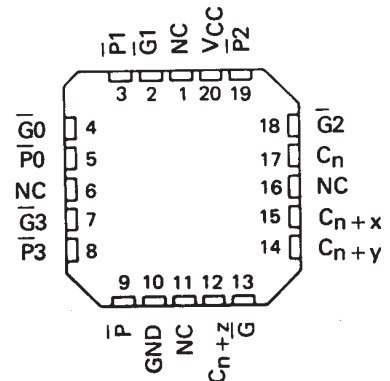
SN54S182 . . . FK PACKAGE (TOP VIEW)
