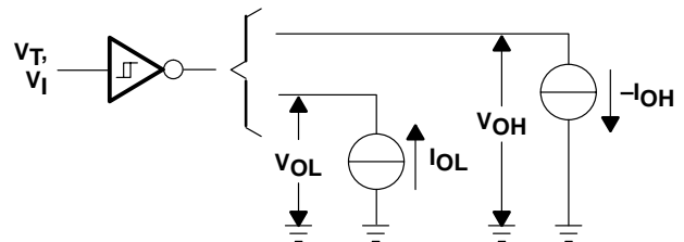
Figure 5. Receiver Test Circuit for V_T , V_{OH} , and V_{OL}
