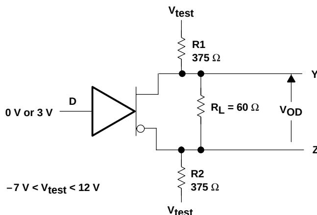
Figure 2. Driver V_{OD}
