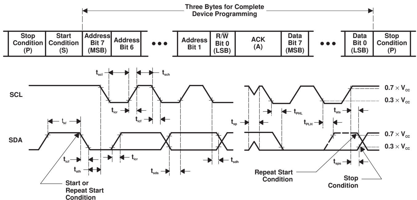
VOLTAGE WAVEFORMS
