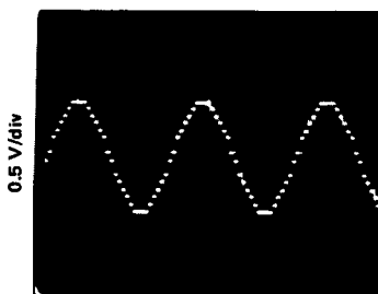
0.2 ms/div
