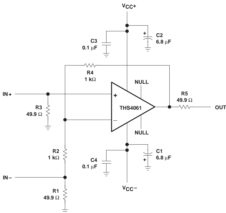
Figure 26. THS4061 Evaluation Board Schematic
