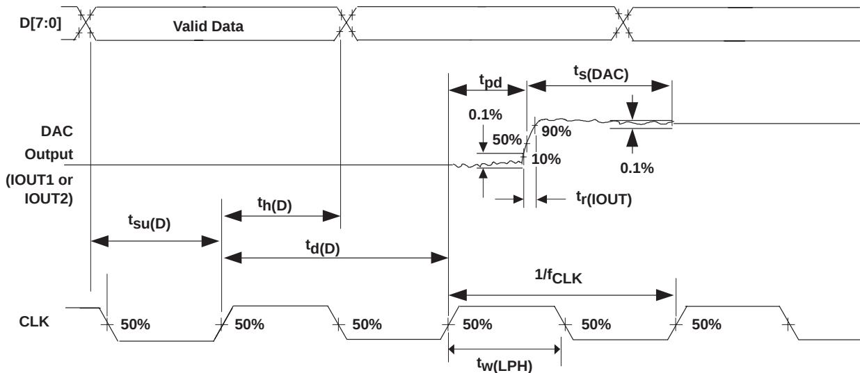
Figure 23. Timing Diagram
