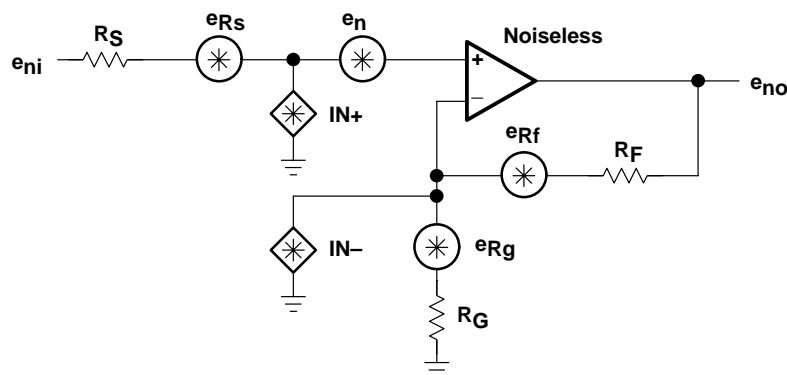
Figure 41. Noise Model
