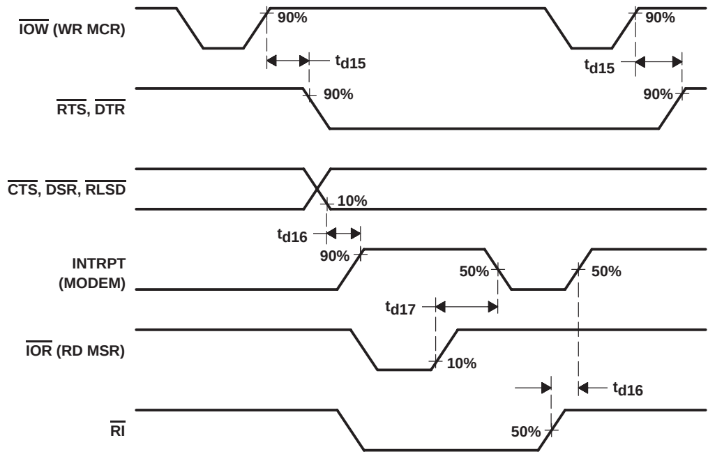
Figure 6. Modem Control Timing Waveforms
