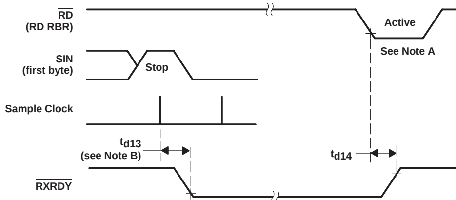
Figure 7. Receiver Ready (RXRDY) Waveforms, FCR0 = 0 or FCR0 = 1 and FCR3 = 0 (mode 0)
