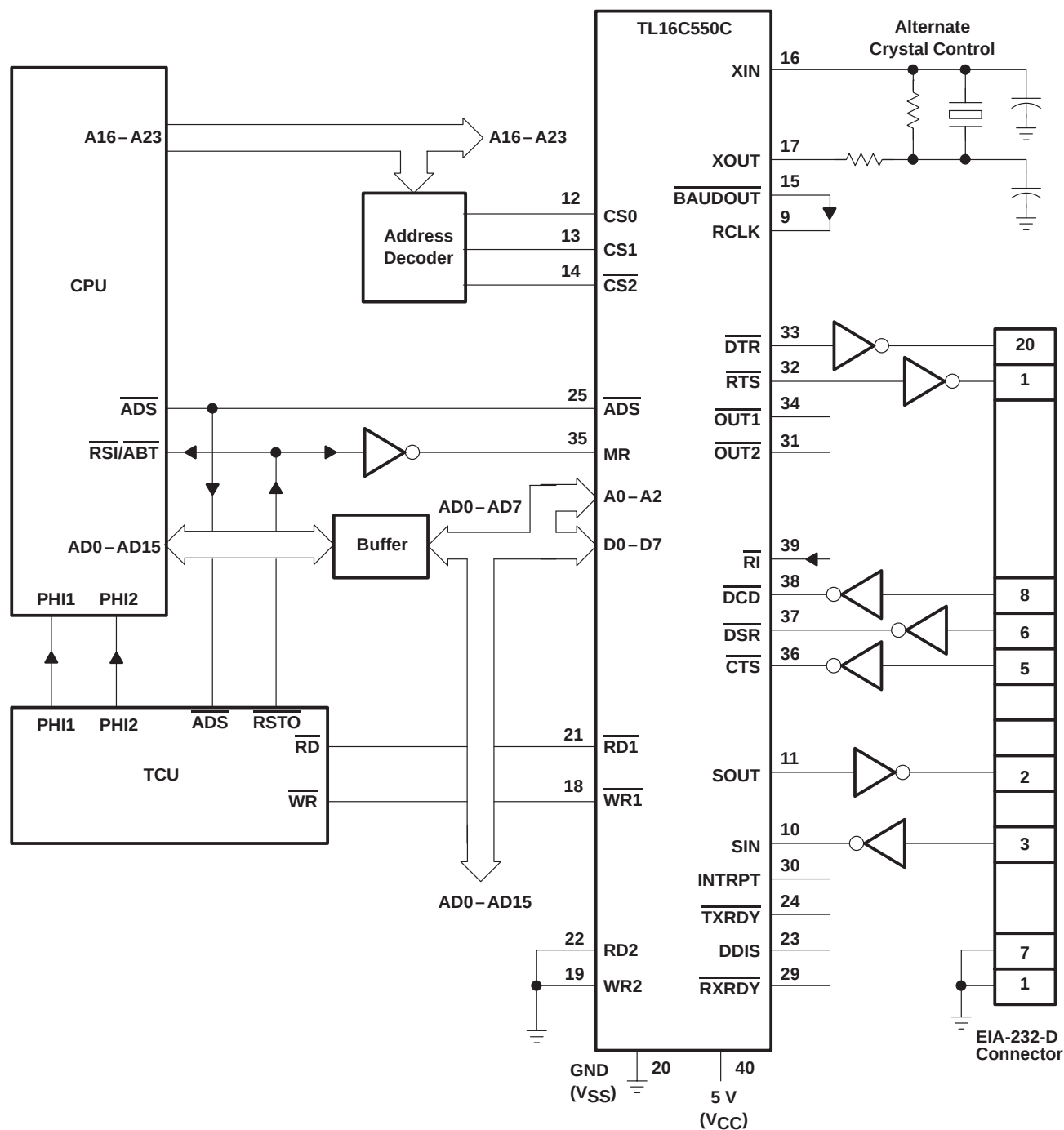
Figure 22. Typical TL16C550C Connection to a CPU
