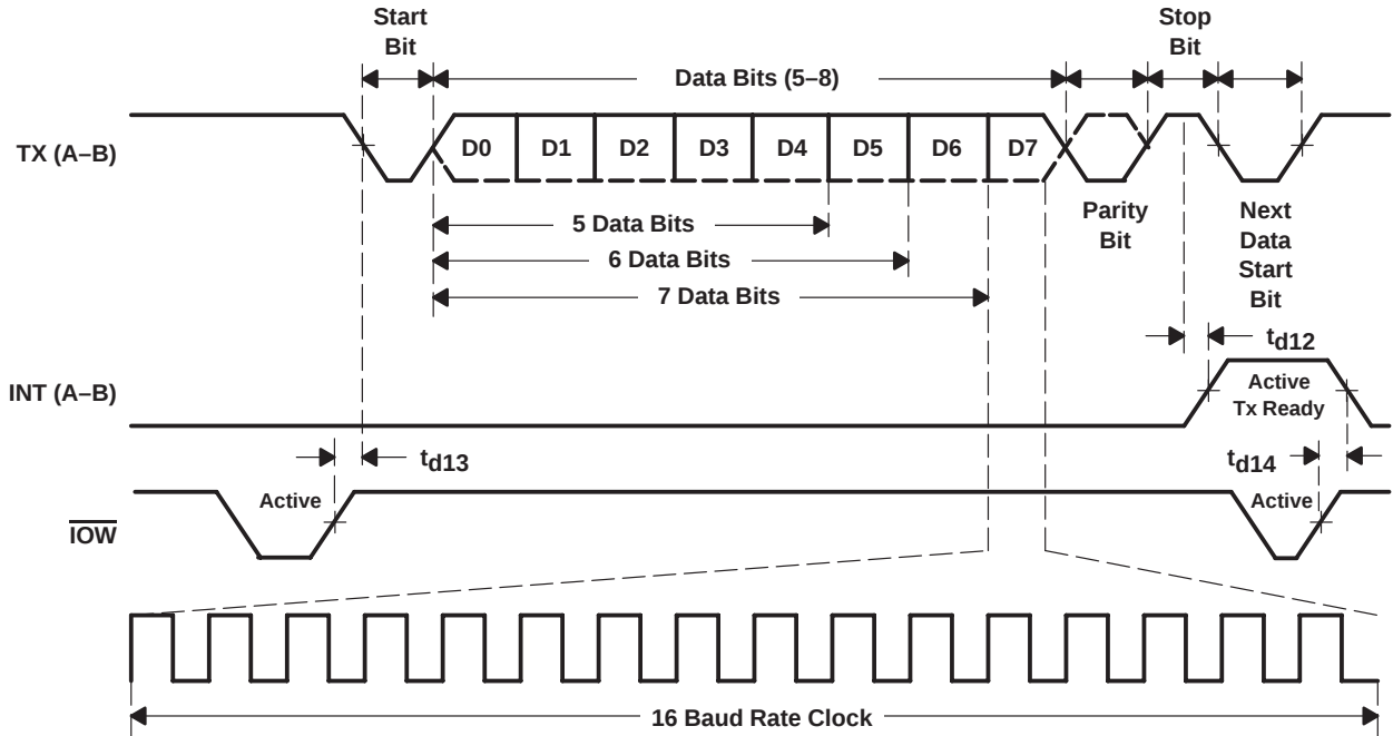
Figure 18. Transmit Timing
