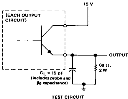
FIGURE 4. EMITTER-FOLLOWER CONFIGURATION
