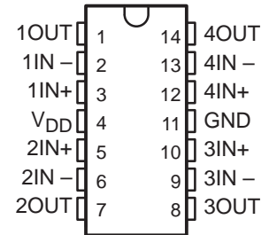
TLC1078 FK PACKAGE (TOP VIEW)
