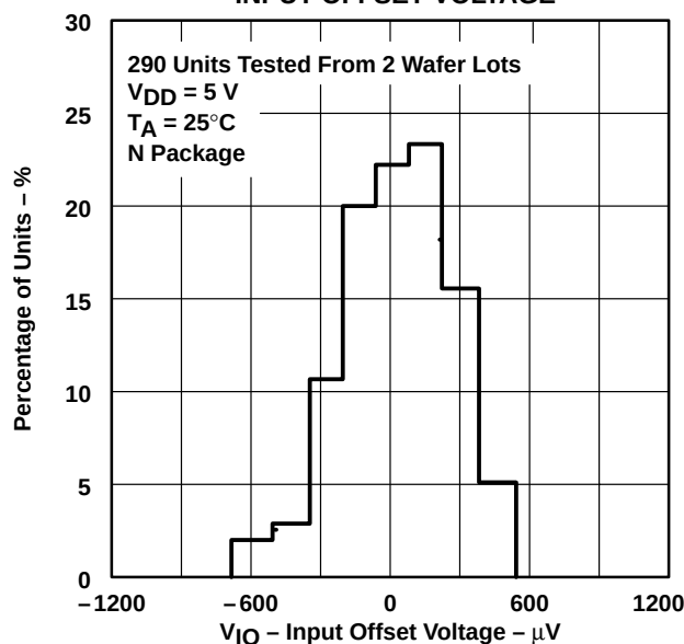
DISTRIBUTION OF TLC279 INPUT OFFSET VOLTAGE
