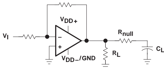
Figure 55. Series-Resistance Circuit
