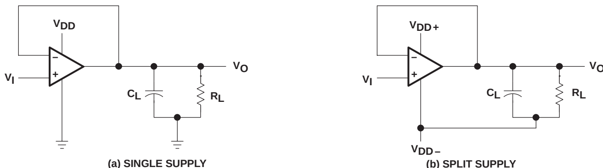
Figure 35. Unity-Gain Amplifier
