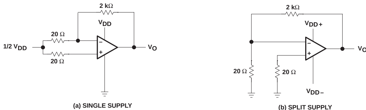
Figure 36. Noise-Test Circuit
