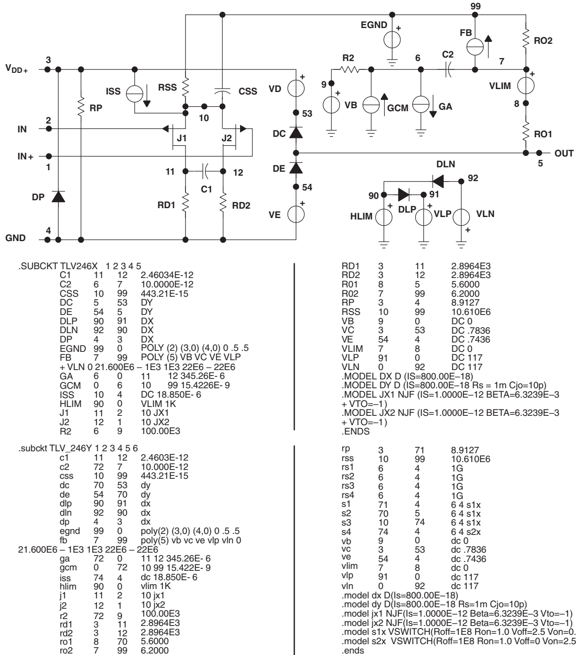
Figure 54. Boyle Macromodel and Subcircuit
