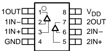
TLV2772 D, DGK, JG, P, OR PW PACKAGE (TOP VIEW)
