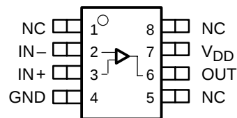
TLV2771 D PACKAGE (TOP VIEW)
