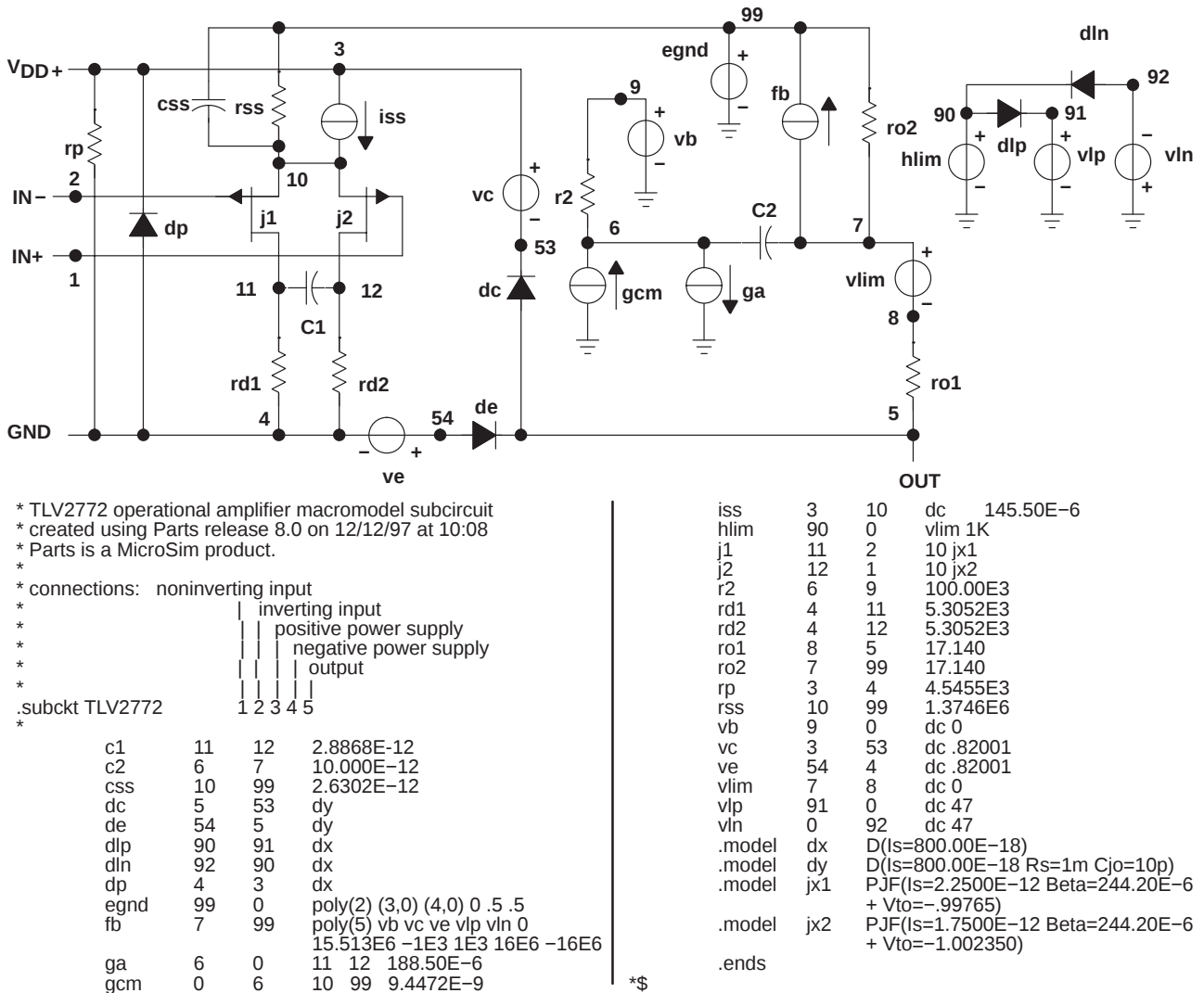
Figure 65. Boyle Macromodel and Subcircuit
