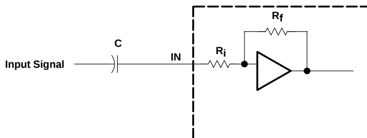
Figure 31. Resistor on Input for Cut-Off Frequency
