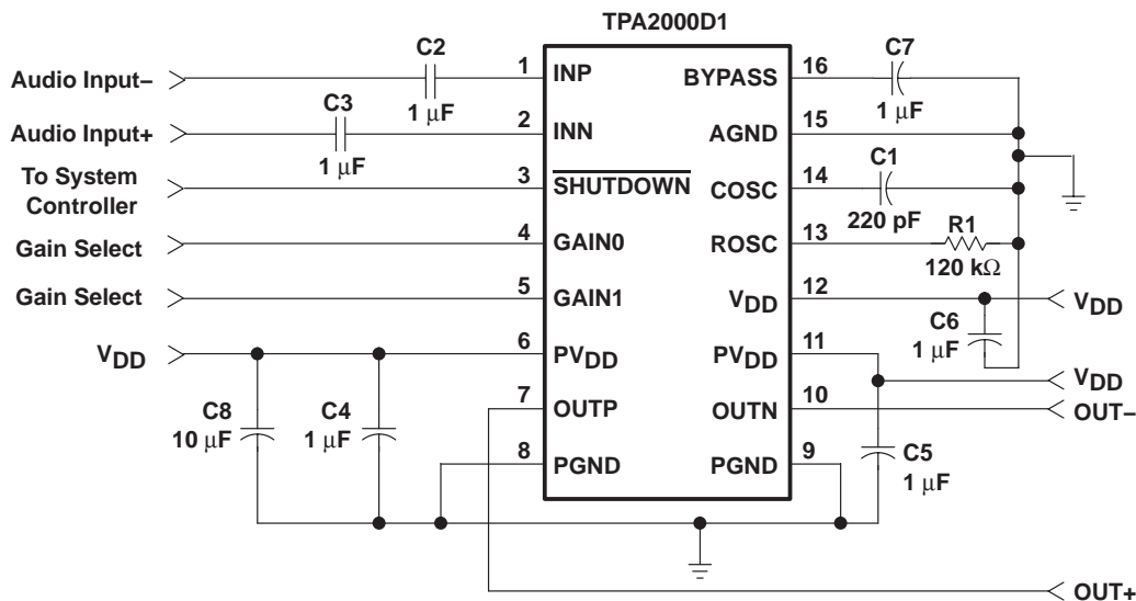
Figure 12. Application Circuit
